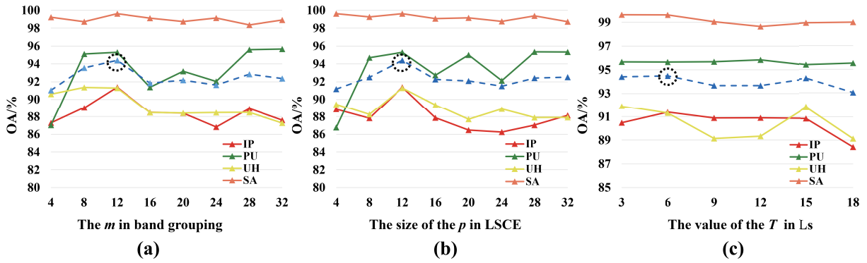
Fig. 9. Effect of different values of MambaLG parameters: (a) m , (b) p , and (c) T on the four datasets.
