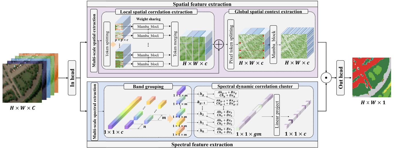
Fig. 2. Flowchart of the proposed MambaLG for HSI classification.
