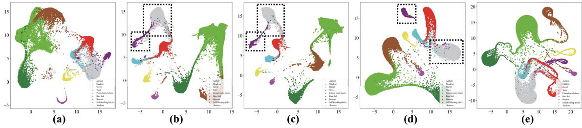
Fig. 10. Visualization of T-SNE results on the PU test samples by different methods, including (a) GSCE, (b) GSCE + MSFE, (c) GSCE + MSFE + LSCE, (d) GSCE + MSFE + LSCE + SpeM, and (e) GSCE + MSFE + LSCE + SpeM + L1.
