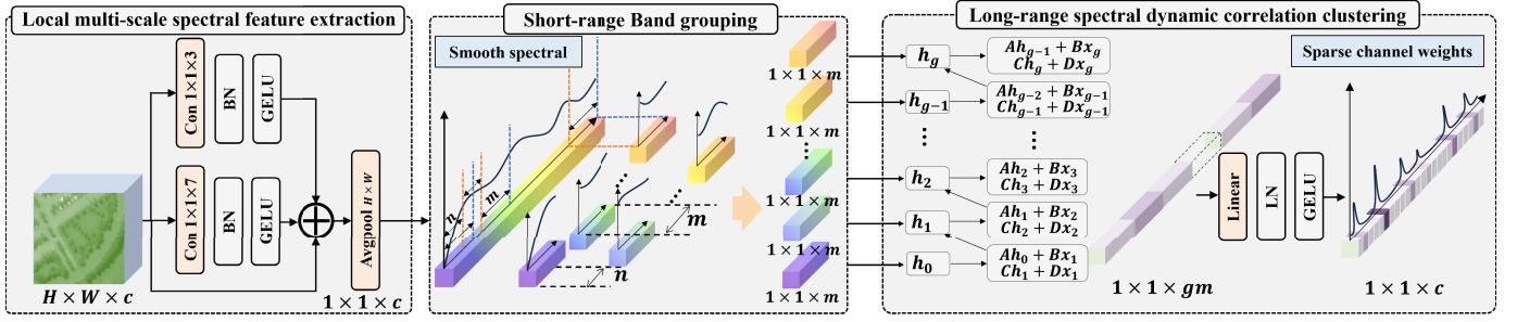
Fig. 4. Illustration of the SpeM for short- and long-range spectral dynamic perception.
