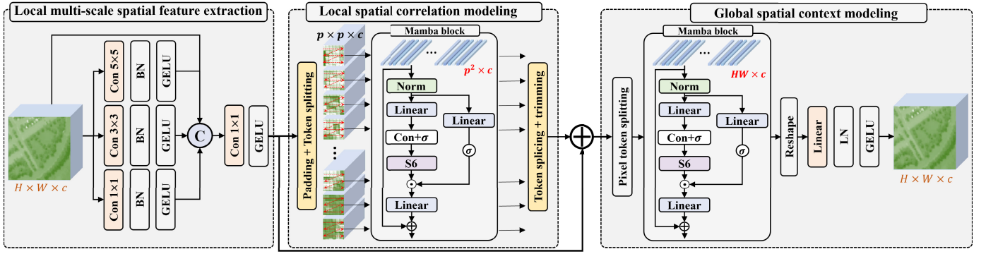
Fig. 3. Graphical illustration of the SpaM for local-to-global spatial semantic modeling.
