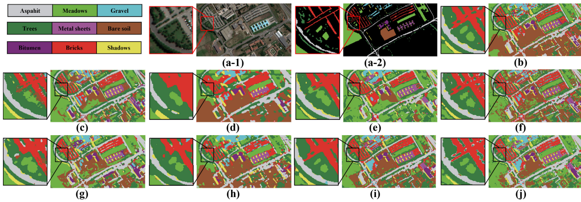
Fig. 6. Visual quality comparison on the PU dataset, which shows the (a-1) pseudocolor image, (a-2) ground truth, and the classification maps corresponding to (b) A2S2K, (c) ASSMN, (d) FDGC, (e) SSDGL, (f) HiT, (g) SSTN, (h) SSFTT, (i) SPRLT, and (j) MambaLG, respectively.
